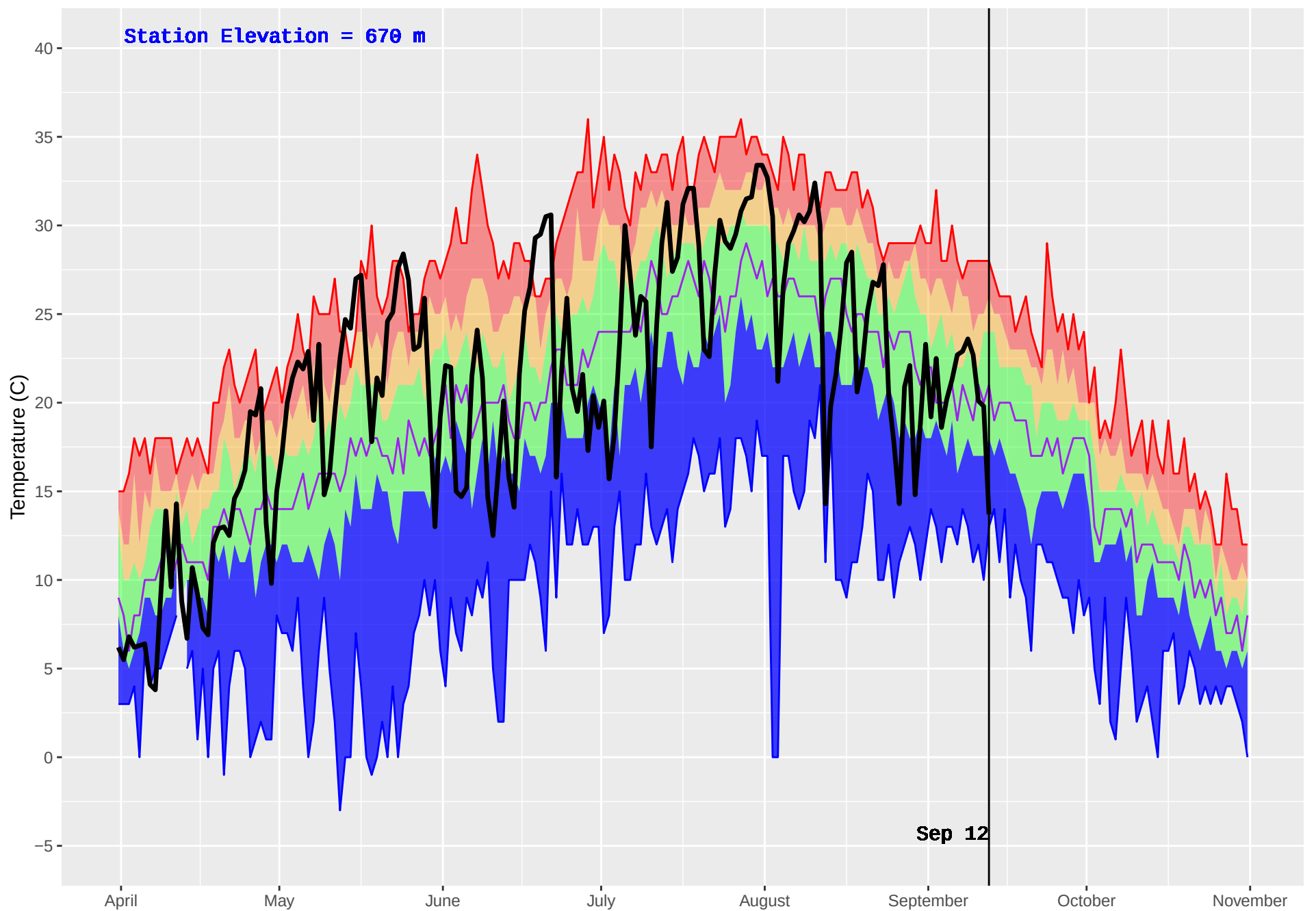
FINTRY (298) : Historical (1989–2016) and Current (2018) Daily Temperature
