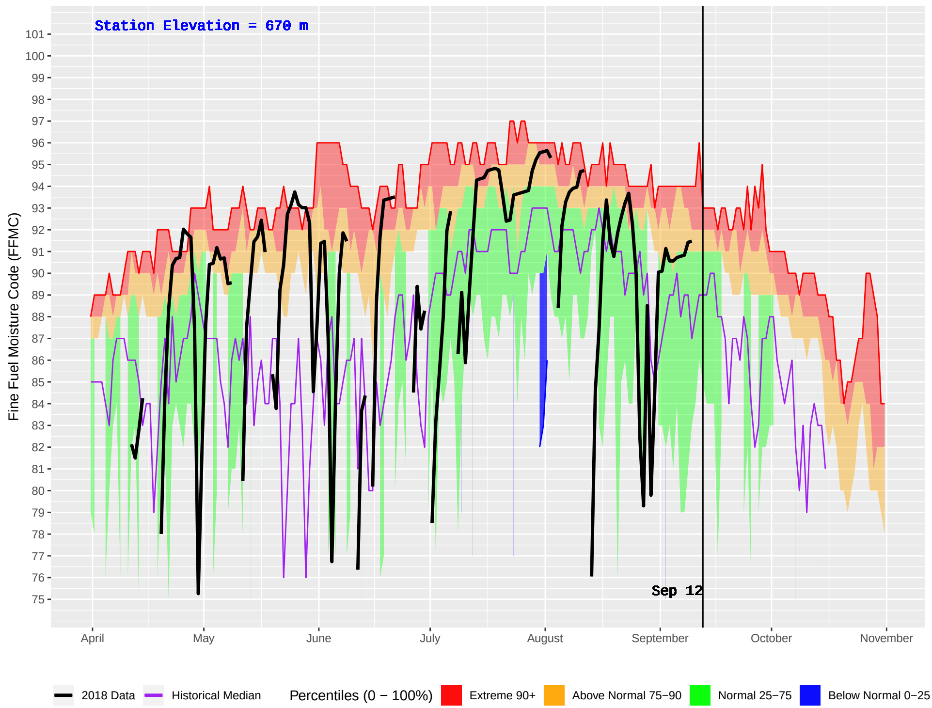
FINTRY (298) : Historical (1989–2016) and Current (2018) Daily Fine Fuel Moisture Code (FFMC)
